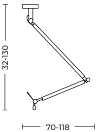
ZYTA S PENDANT LAMPBODY AZ2298
