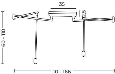
NATALIA 2S LAMPBODY AZ1923
