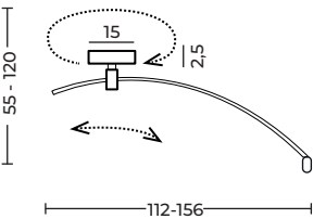
SELENA 2 LAMPBODY AZ2284
