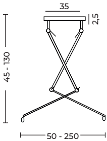
ADAM 2S LAMPBODY AZ1842
