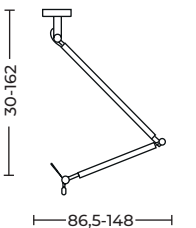
ZYTA M PENDANT LAMPBODY AZ1847
